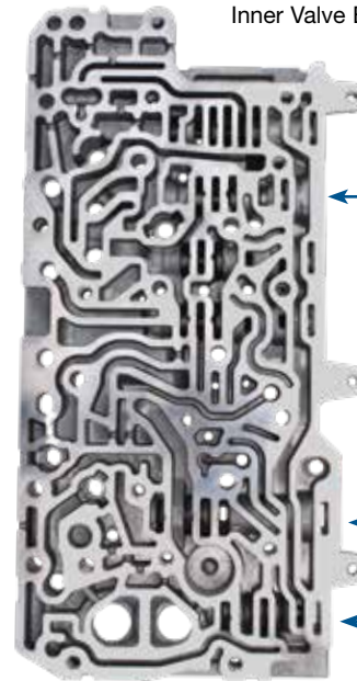
ZF9HP48 PBC Inner Valve Body
