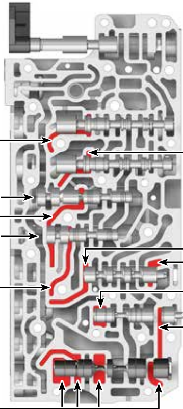
Lower Valve Body
