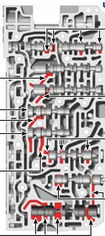
Lower Valve Body
