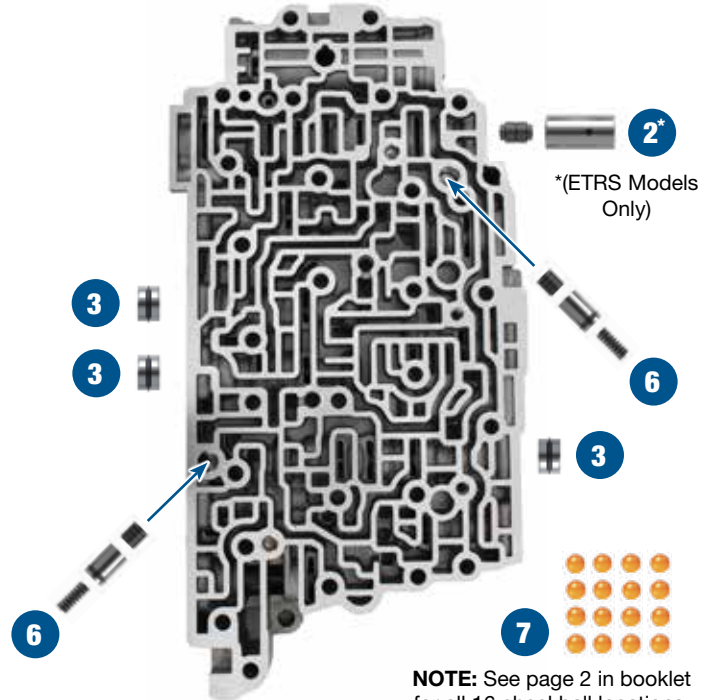
9T50 Main Control Valve Body
