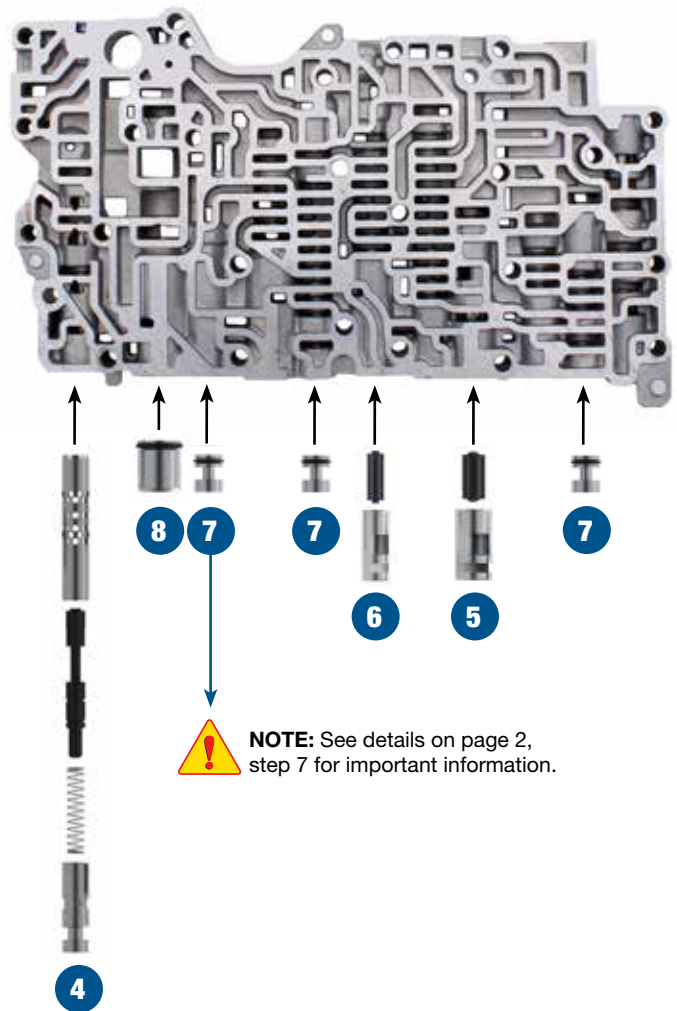
UB80E Middle Valve Body
