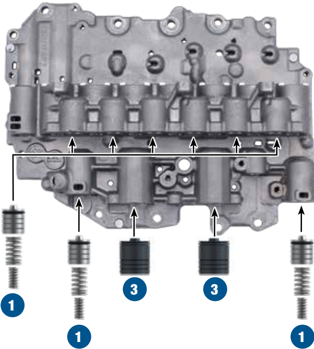
UB80E Solenoid Valve Body
