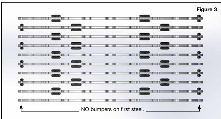
Rubber Bumper
