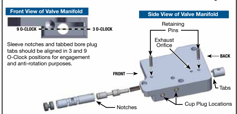
Valve Assembly Installation into Valve Manifold Figure 6
