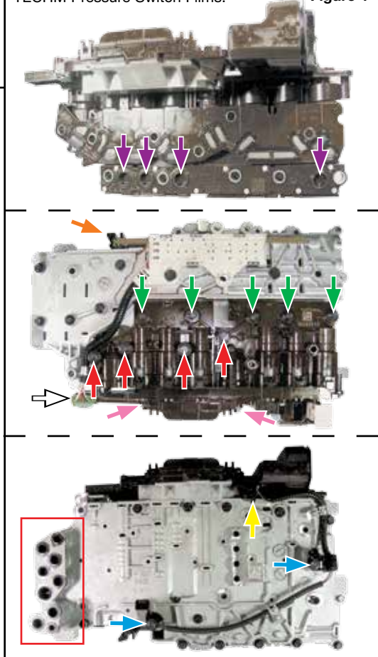
TECHM Pressure Switch Films. Figure 1
